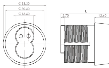
Taper Head Mortise Cylinder W/IC Core
