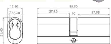
Euro Profile Oval Double Cylinder W/ I.C Core
