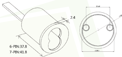
Rim Cylinder For Panic Device W/ IC Core
