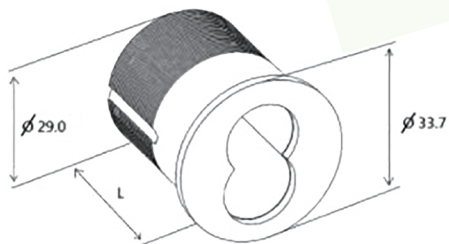
Mortise Cylinder W/ IC Core
