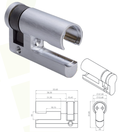
Euro Profile Half Cylinder W/ I.C Core
