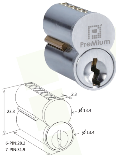
Small Format Interchangeable Core Cylinder (SFIC)
