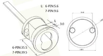
Rim Cylinder W/IC Core
