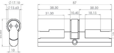
Euro Profile Double Cylinder W/ I.C Core
