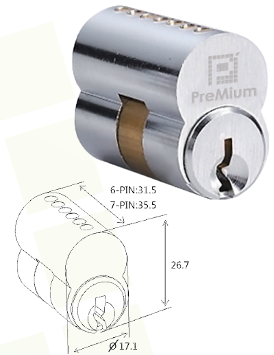
Large Format Interchangeable Core (LFIC)
