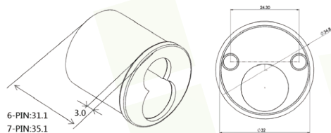
Rim Cylinder W/ IC Core
