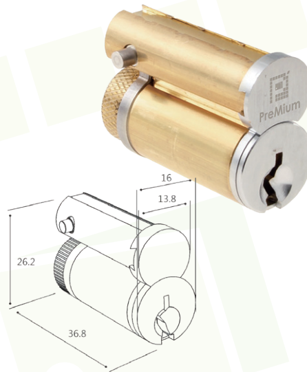
Schlage Large Format Interchangeable Core (LFIC)
